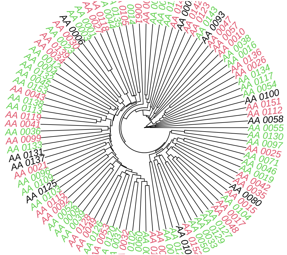
UPGMA Tree (Bray-Curtis) by Age Group
